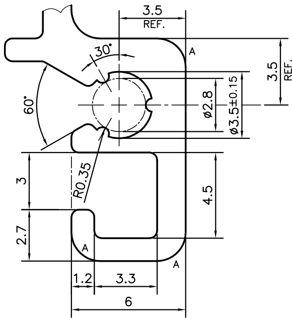
DETAIL OF "A" SCALE- 5:1
