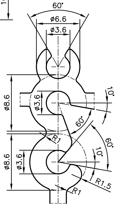
DETAIL OF "A" SCALE 3:1
