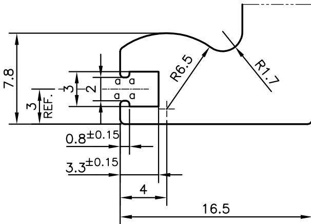
DETAIL OF "A" SCALE 3:1
