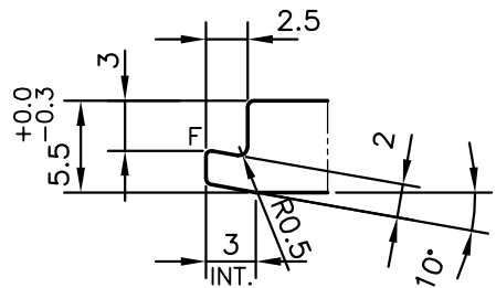
DETAIL OF "B" SCALE 2:1
