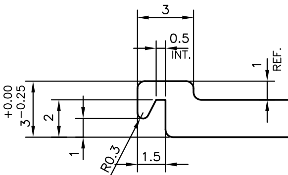
DETAIL OF "A" SCALE 5:1
