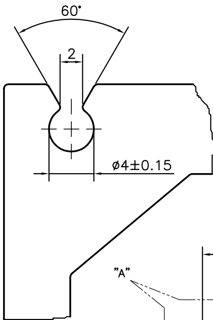
DETAIL "A" SCALE 3:1
