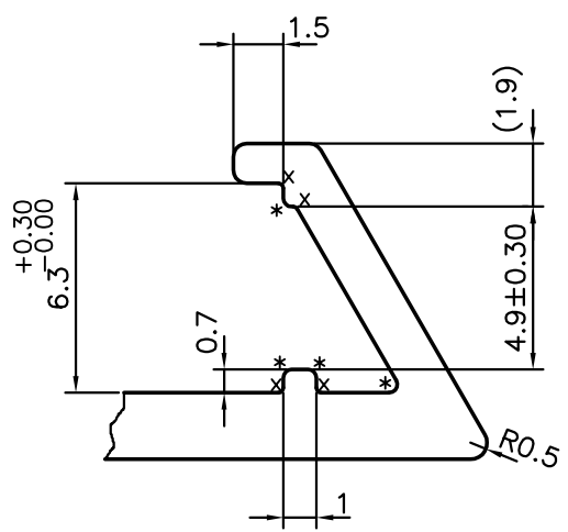
DETAIL OF "A" SCALE 4:1
