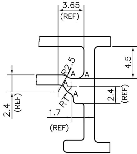
DETAILS OF "X" SCALE 3:1
