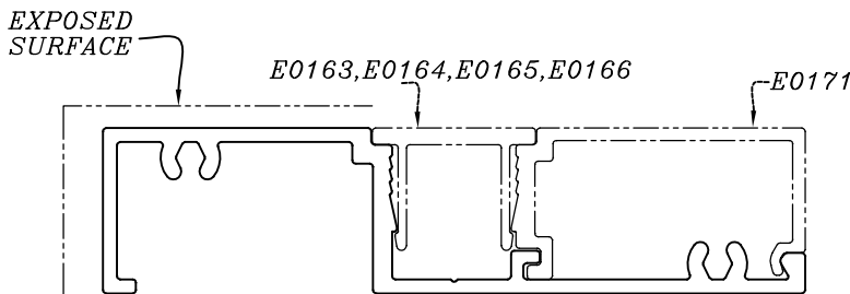
DETAIL OF "B" SCALE 2:1
