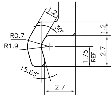
DETAIL OF "A" SCALE 6:1
