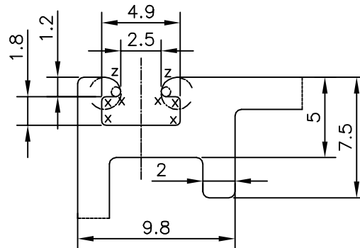
DETAIL OF "B" SCALE 2:1
