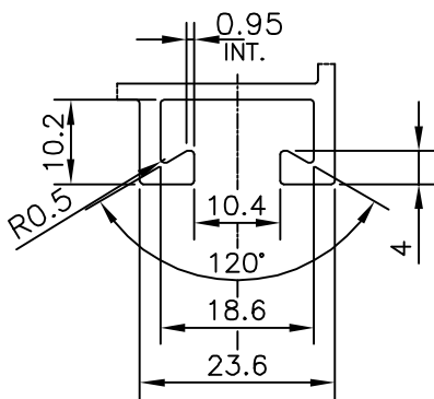
DETAIL OF "A" SCALE 1:1
