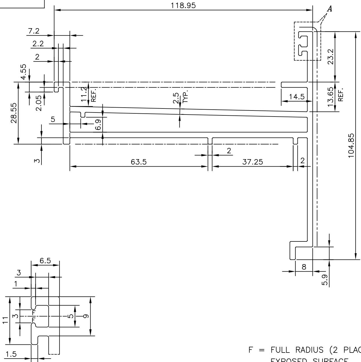
DETAIL OF "A" SCALE 2:1
