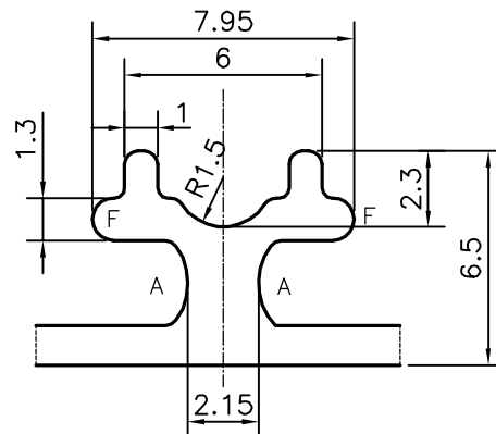
DETAIL OF "B" SCALE 4:1
