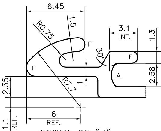
DETAIL OF "A" SCALE 4:1
