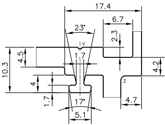
DETAIL OF "A" SCALE 3:1
