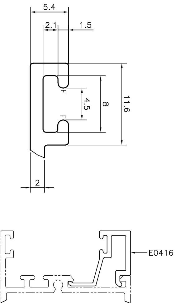
DETAIL OF 'A' SCALE 3:1
