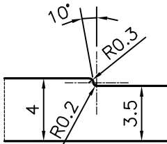
DETAIL OF "A" SCALE 3:1
