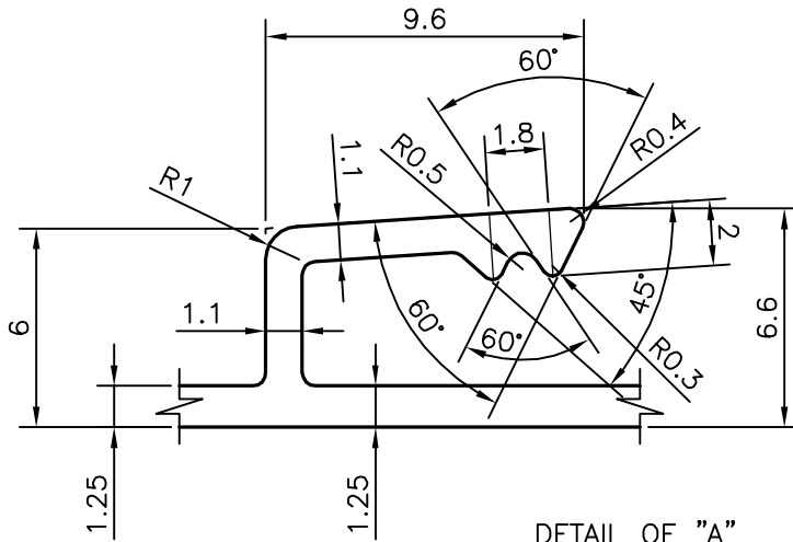
DETAIL OF "A" SCALE 4:1
