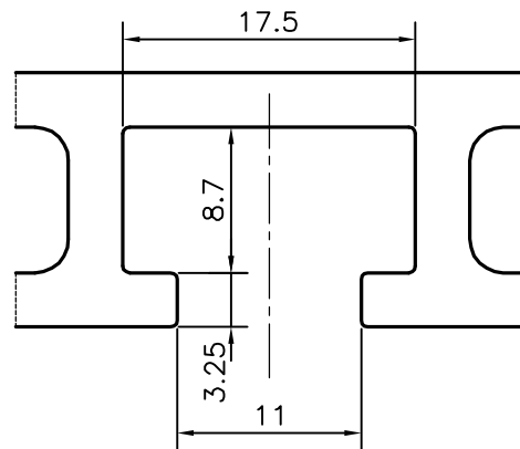
DETAIL OF "B" SCALE 2:1
