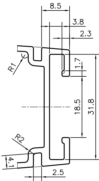
DETAIL OF "A" SCALE 1.5:1
