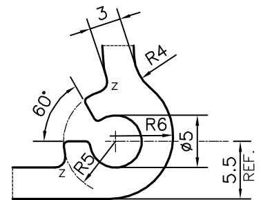
DETAIL OF "C" SCALE 2:1
