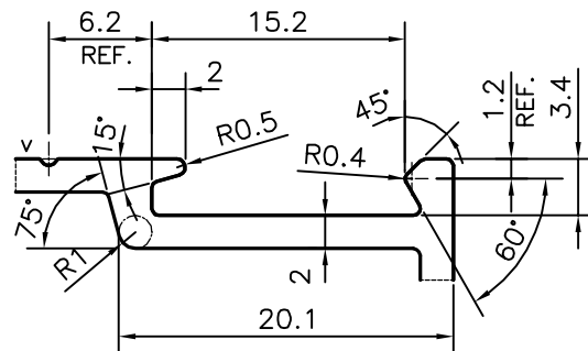
DETAIL OF "A" SCALE 2:1
