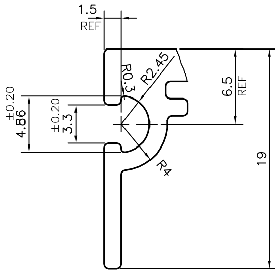
DETAIL "A" SCALE 3:1
