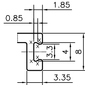
DETAIL OF "A" SCALE 2:1
