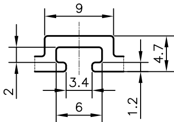
DETAIL OF "A" SCALE 2:1
