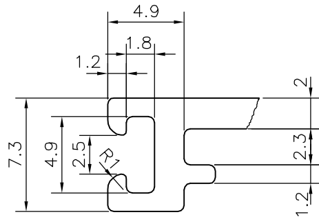
DETAIL OF "A" SCALE 3:1
