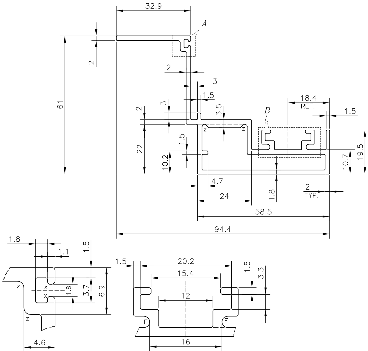
DETAIL OF "A" SCALE 3:1
