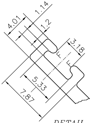
DETAIL OF "A" SCALE 3:1
