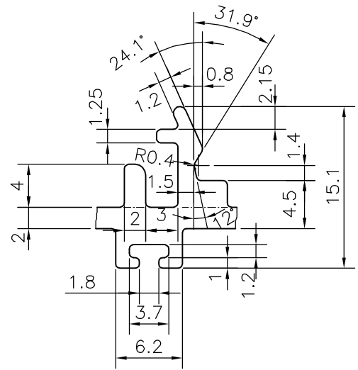
DETAIL OF "B" SCALE 2:1
