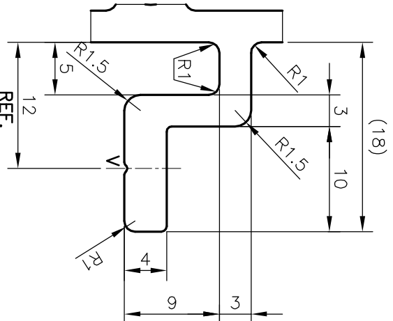
DETAIL OF "C" SCALE 2:1
