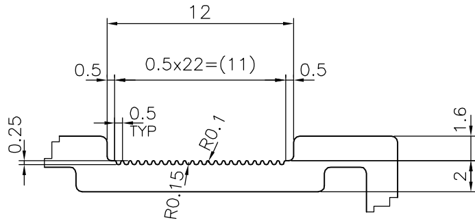
DETAIL OF "A" SCALE 3:1
