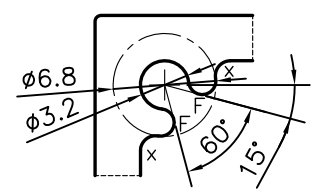
DETAIL OF "A" SCALE 2:1
