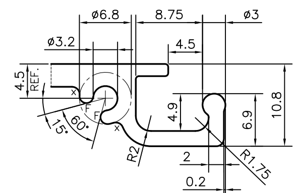
DETAIL OF "C" SCALE 2:1
