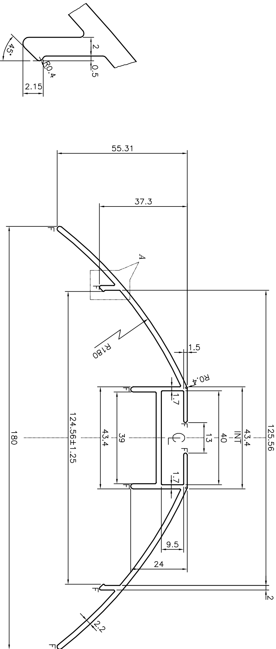
DETAIL OF "A" SCALE 4:1
