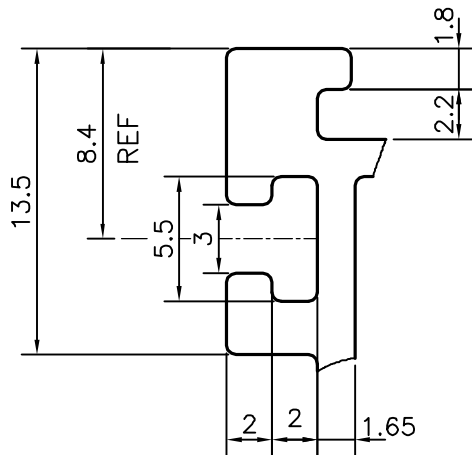
DETAIL OF "A" SCALE 3:1
