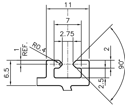
DETAIL OF "A" SCALE 2:1
