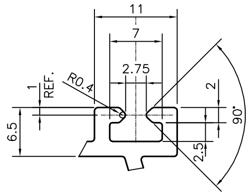
DETAIL OF "A" SCALE 2:1
