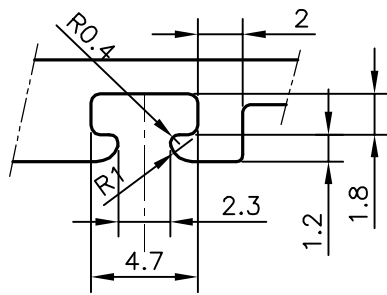
DETAIL OF "A" SCALE 3:1
