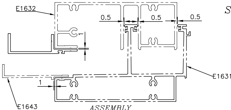
ASSEMBLY SCALE 1:2
