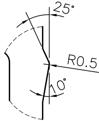
DETAIL B SCALE 3:1
