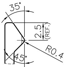
DETAIL A SCALE 3:1
