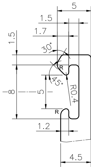
DETAIL B SCALE 3:1
