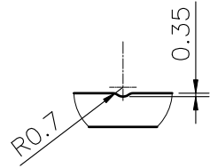
DETAIL G (7 PLACES) SCALE 2:1
