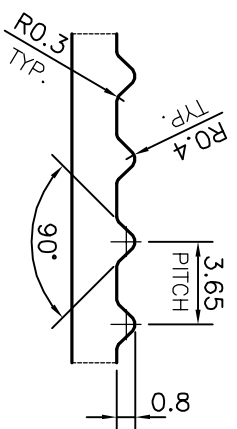
DETAIL OF "A" SCALE 3:1 TYP. DETAIL
