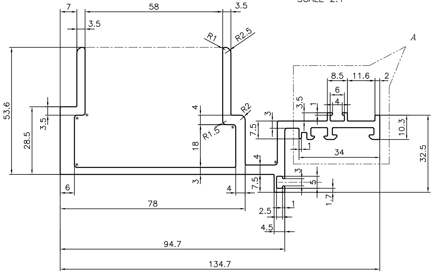
DETAIL OF "A" SCALE 2:1
