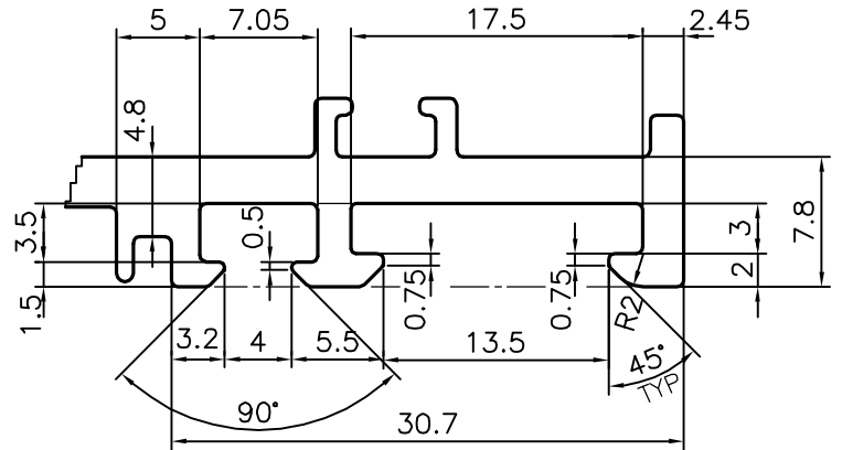
DETAIL OF "A" SCALE 2:1
