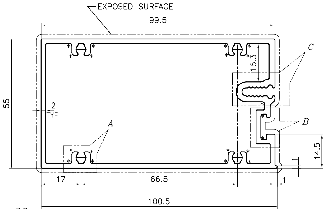
DETAIL OF "B" SCALE 2:1
