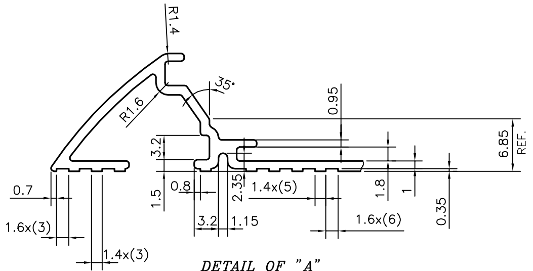
DETAIL OF "A" SCALE 2:1
