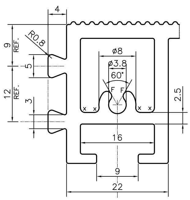
DETAIL OF "B" SCALE 2:1
