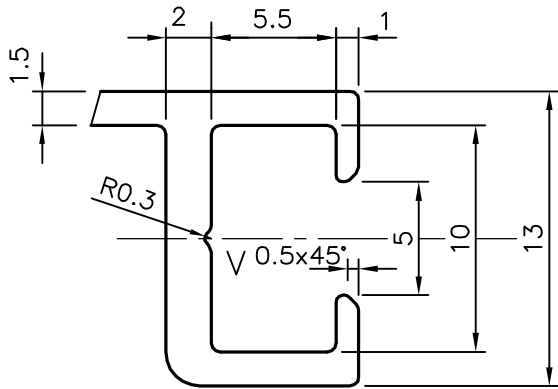
DETAIL-B SCALE 3:1
