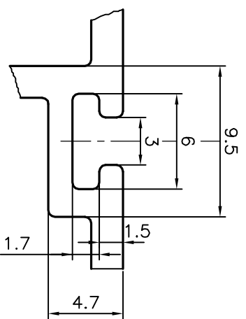
DETAIL OF "B" SCALE 3:1
