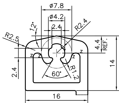
DETAIL OF "C" SCALE 2:1
