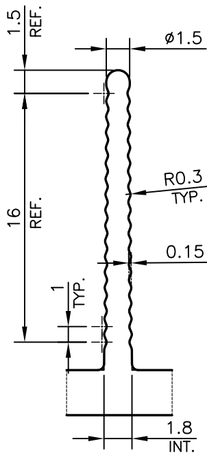
DETAIL OF "A" SCALE 3:1
