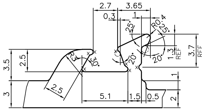
DETAIL OF "A" SCALE 4:1
