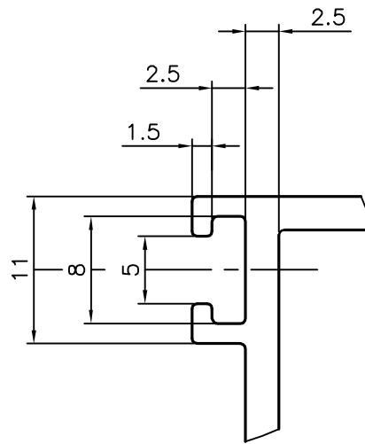
SCALE 2:1 DETAIL OF "B"
