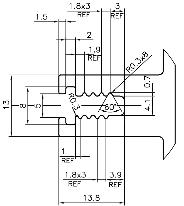
SCALE 2:1 DETAIL OF "A"
