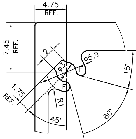
DETAIL OF "A" SCALE 3:1
