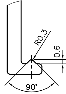
DETAIL OF "B" SCALE 3:1
